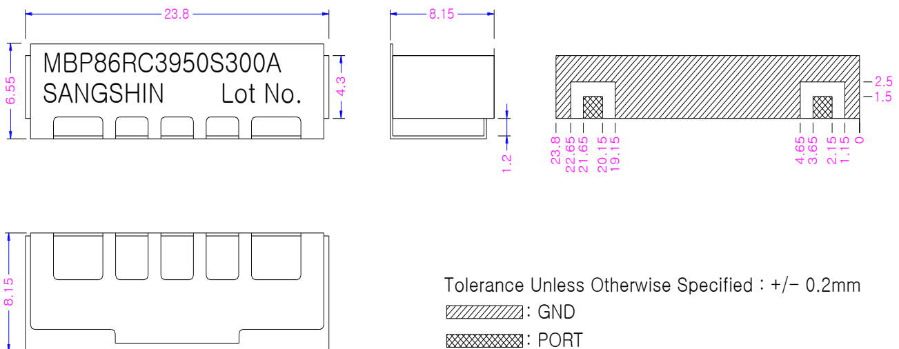
Top View
